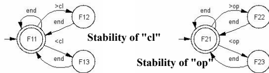
Fig. 7 Stability of the outputs
