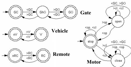
Fig. 3 Plant Model of the automatic gate
