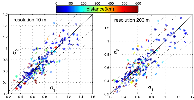
Figure 4. Scatter plot of rms of relative temperature fluctuations (in K) in collocated radiosonde profile pairs. The color denotes horizontal separation (distance with respect to air d_{air} ) of measurements. (left) Profiles are in original resolution; (right) profiles are smoothed down to 200 m vertical resolution. Solid line, y=x ; dashed lines, y=1.2x and y=(1/1.2)x ; dotted lines, y=1.4x and y=(1/1.4)x .
