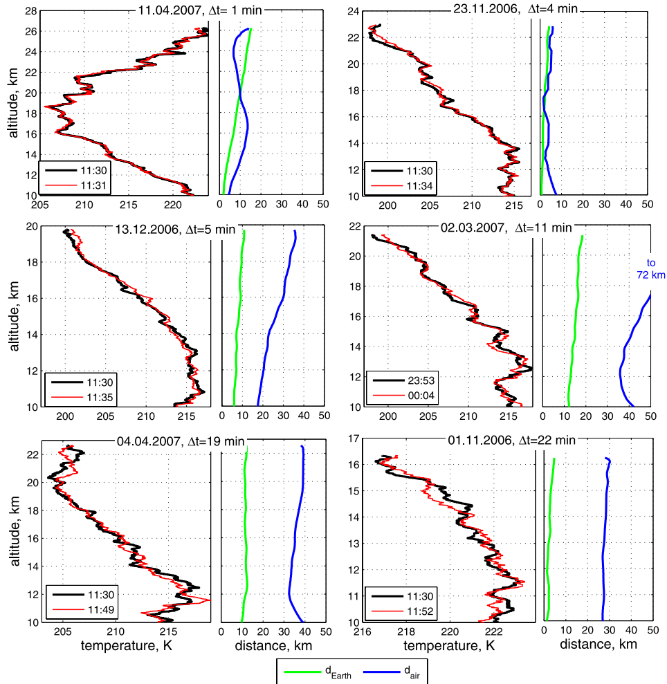
Figure 1. (left) Examples of Sodankylä radiosonde temperature profiles corresponding to small time difference between sonde launches. (right) Distances with respect to Earth d_{Earth} and with respect to air d_{air} .
