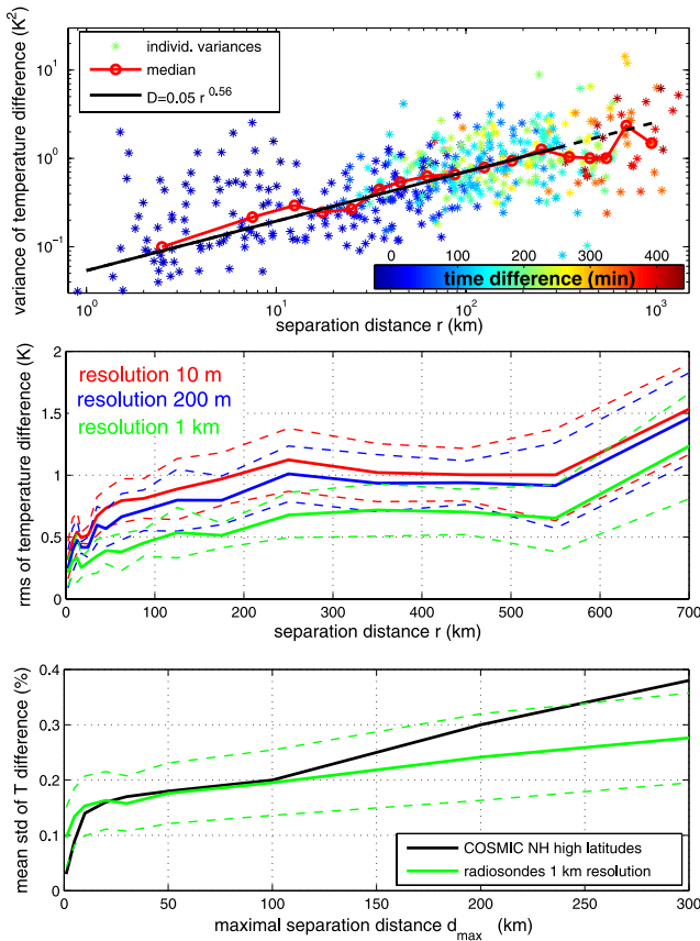
Figure 2. (top) Experimental estimates of the structure function D_T(r) (equation (1)), stars: D_T(r) values computed using collocated profile pairs, the color indicates time difference; red line: median \langle D_T(r) \rangle , circles mark the mid points of the bins used for data averaging; black line: the fit by the power function. Only data with r < 300 km were used in the fit (solid line), the extension of the fit to r > 300 km is indicated by dashed black line. (middle) Rms of temperature difference in collocated profiles as a function of separation distance, on a linear scale, calculated using the above-mentioned bins, Solid lines: median, dashed lines: inter-quartile range. Red: original resolution ( \sim 10 m), blue: vertical resolution 200 m, green: vertical resolution 1 km. (Red lines represent the same data in top and middle subplots). (bottom) Mean std of temperature/refractivity difference (in %) for profiles pairs with the separation distance smaller than d_{max} , presented as a function of d_{max} . The black line shows the COSMIC data for the Northern Hemisphere high latitudes adapted from Anthes et al. [2008].
