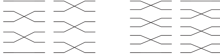
Figure 3: s_{\text{even}} and s_{\text{odd}} for n = 6, 7 .
