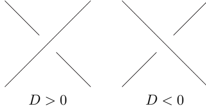
Figure 6: The two cases of crossings
