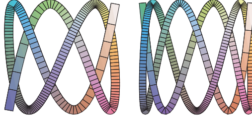
Figure 10: The torus knots 5_1: H(3, 7, 8) and 7_1: H(3, 10, 11)
