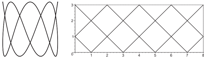
Figure 2: T_8(x) = T_3(y) and its billiard picture
