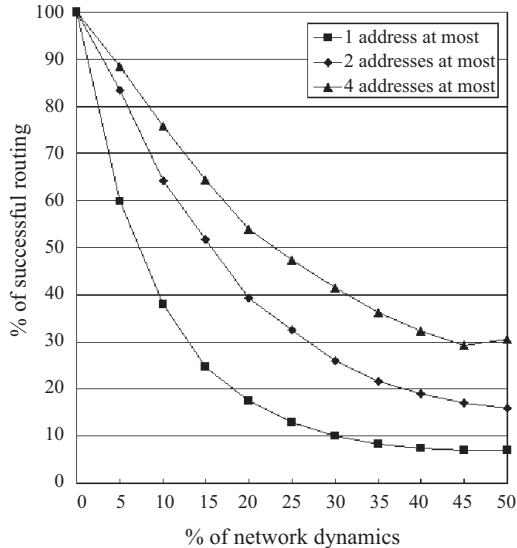
Fig. 11. Percentage of success vs. network dynamics.
