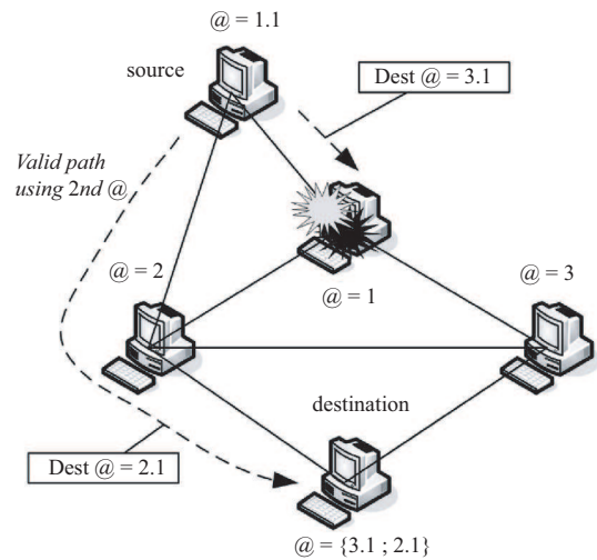
Fig. 4. Alternate routing for solving network dynamics.
