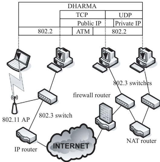
Fig. 8. Network convergence with our middleware.
