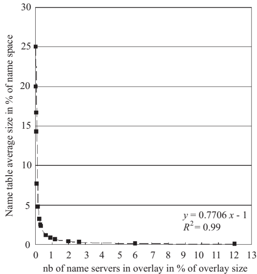
Fig. 17. Name table size vs. number of name servers.
