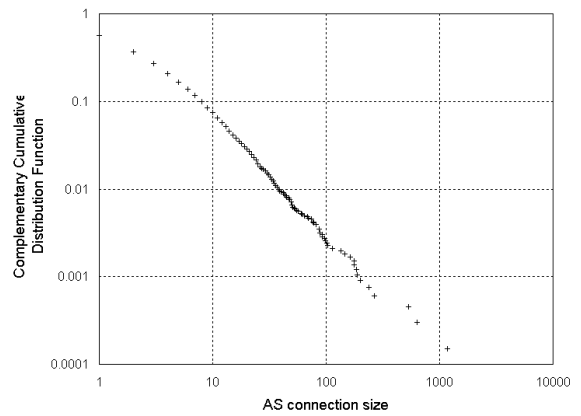
Fig. 4. BGP connection size CCDF.
