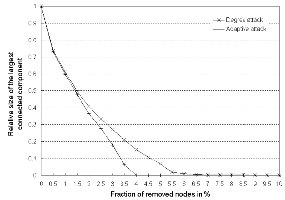
Fig. 6. LSIIIT'02 largest cluster size evolution.
