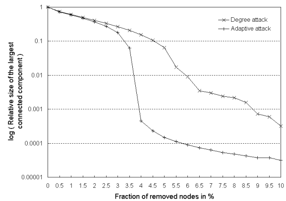
Fig. 8. LSIIIT'02 largest cluster size evolution (log scale).
