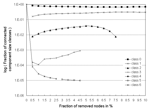
Fig. 12. Cluster class fraction (adaptive attack, log scale).
