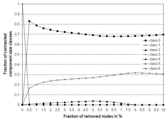
Fig. 10. Cluster class fraction (adaptive attack).
