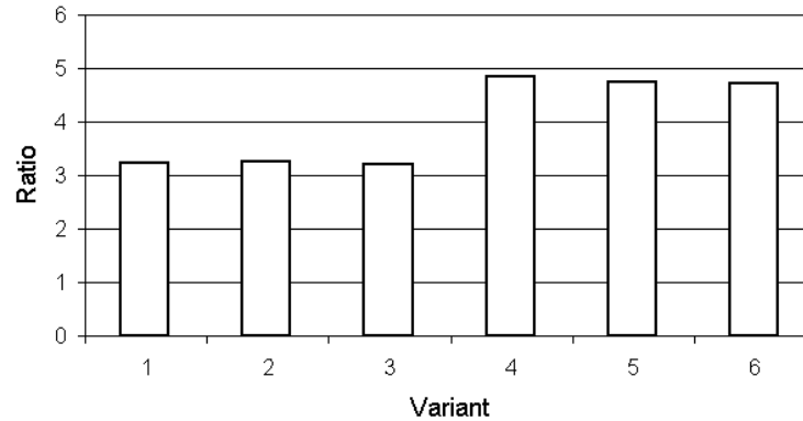
Fig. 6: Routers involved
