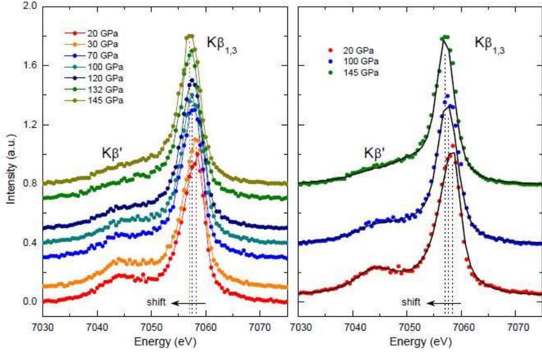
FIG. 31 (Color online) a) Fe X-ray emission spectra measured in (\text{Mg}_{0.9}\text{Fe}_{0.1})\text{SiO}_3 between 20 and 145 GPa; b) XES spectra in model compounds (solid lines) are superimposed on to three spectra representative of the three different spin states. From Badro et al. (2004).
