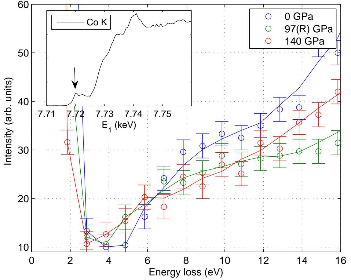
FIG. 25 (Color online) RIXS in CoO as a function of pressure (open circles); lines are 3-point average of the data; the incident energy is tuned to the quadrupolar pre-peak in the absorption spectrum (arrow in inset). (R) indicates pressure release.
