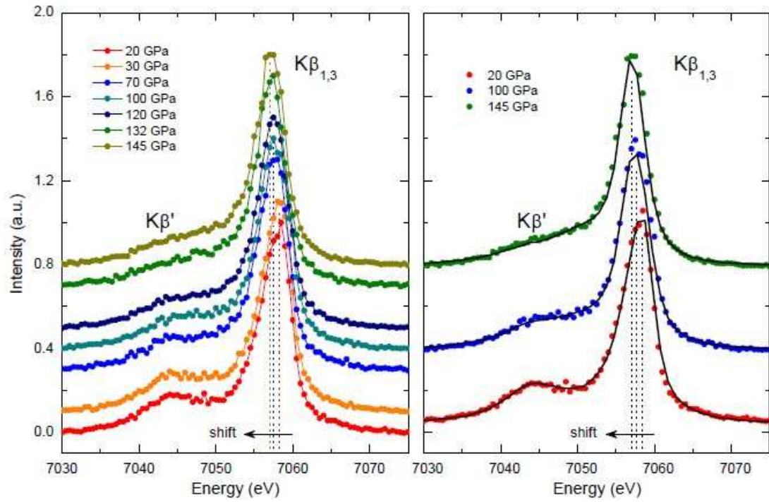
FIG. 31 (Color online) a) Fe X-ray emission spectra measured in (\text{Mg}_{0.9}, \text{Fe}_{0.1})\text{SiO}_3 between 20 and 145 GPa; b) XES spectra in model compounds (solid lines) are superimposed on to three spectra representative of the three different spin states. From Badro et al. (2004).
