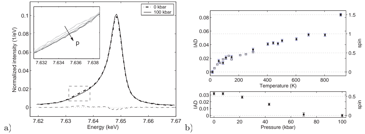
FIG. 32 a) Evolution of the K \beta emission line in LaCoO _3 as a function of pressure; b) Pressure ( T = 300 K) and temperature (at ambient pressure) dependence of IAD values derived from XES (left scale) and estimated Co spin-state (right scale). From Vankó et al. (2006b).
