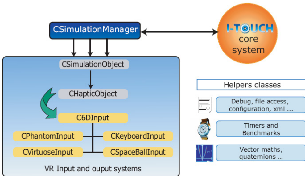
Figure 1: I-Touch framework architecture.
