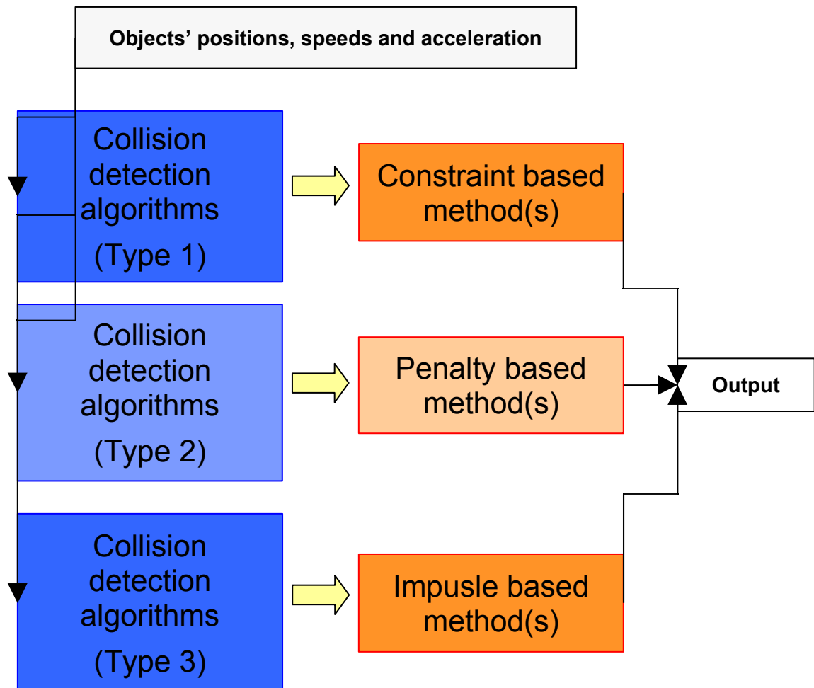
Figure 2: I-Touch interaction between collision detection and response
