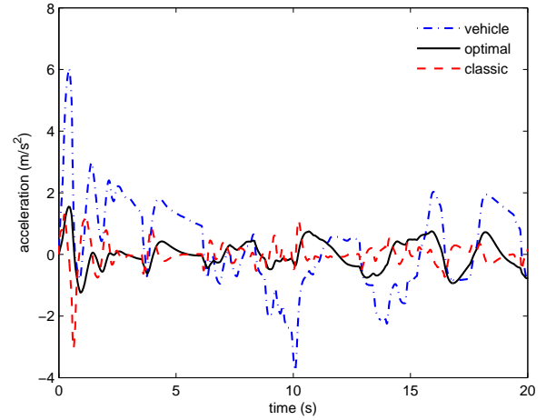
Fig. 19. Acceleration response comparison according to classical and optimal algorithms.
