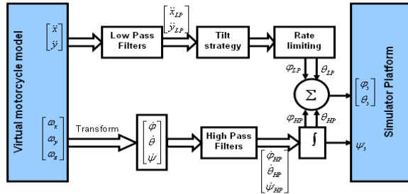
Fig. 5. Motion Cueing strategy
