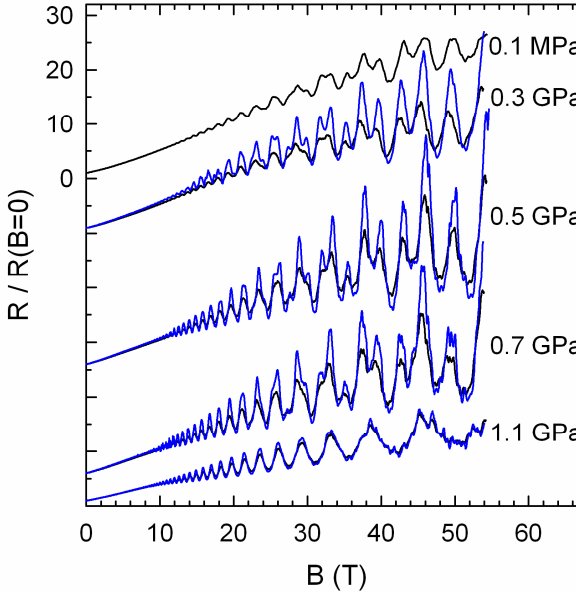
Fig. 3. (color on line) Field-dependent interlayer resistivity at various applied pressures. Curves have been shifted by an arbitrary amount for clarity. Black and blue solid lines correspond to data measured at 4.2 K and 1.7 K, respectively.
