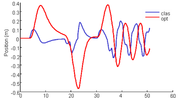
Fig. 12. Cabin's positions using optimal and classical algorithms
