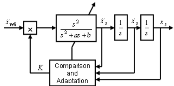
Fig. 4. Adaptive Washout Algorithm for longitudinal displacement
