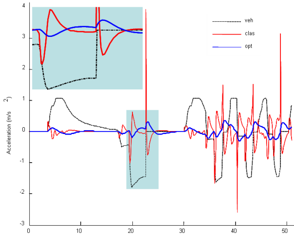
Fig. 10. Cabin's accelerations using optimal and classical algorithms
