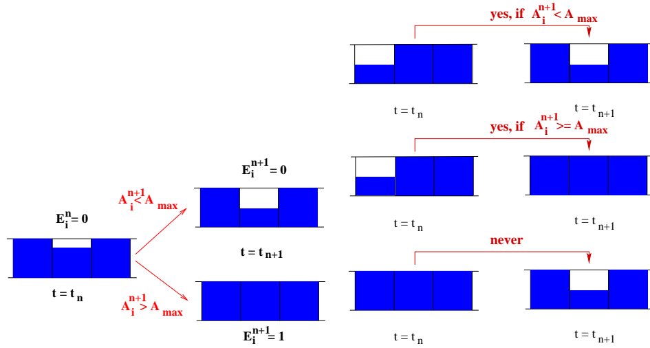
Figure 9: Update of the state E_i^{n+1} of the mesh m_i .
