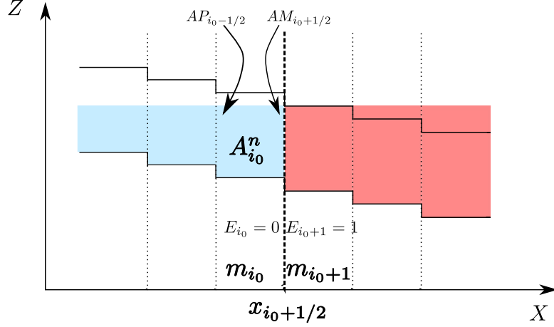
Figure 11: Discrete representation of the mixed free surface-pressurized still water steady state at time t^n .
