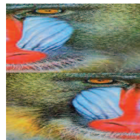
Figure 4: Third step of the BT initial iteration ( 256 \times 256 ).
