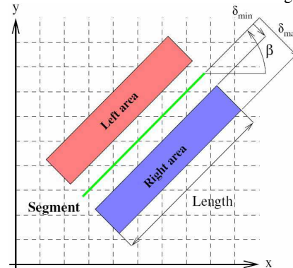
Figure 3. Line segment vicinity.
