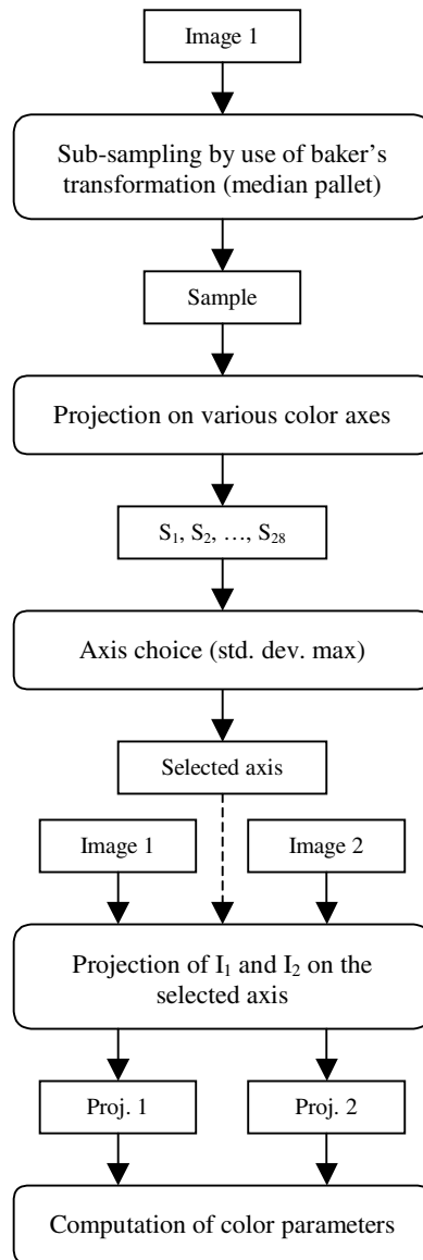
Figure 6. Sub-process for computation of color parameters.
