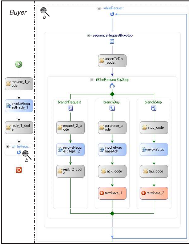
Fig. 2. WF workflow for the Buyer component
