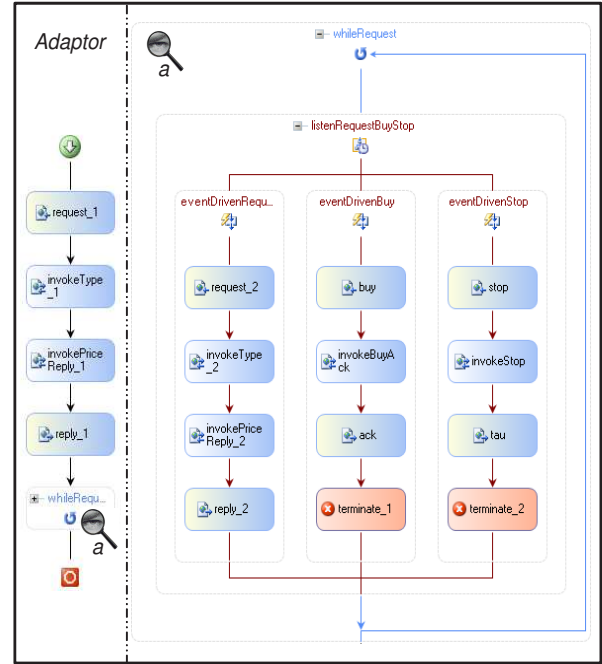
Fig. 5. WF workflow for the Adaptor component
