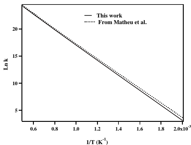
Figure 3: Comparison between of the rate constant for the reaction c\text{-C}_4\text{H}_7 \rightarrow \text{C}_4\text{H}_7 calculated at the CBS-QB3 level (this work) and that of Matheu et al. 9 , at the CBS-Q level of theory.
