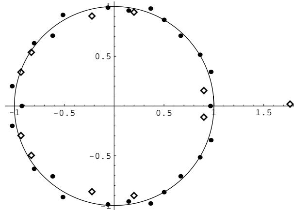
Figure 3. Concentration and equi-distribution of the Galois conjugates ( \diamond ) \neq \beta and the beta-conjugates ( \bullet ) of the second-smallest NR Pisot number \beta = 1.764\dots near the unit circle.
