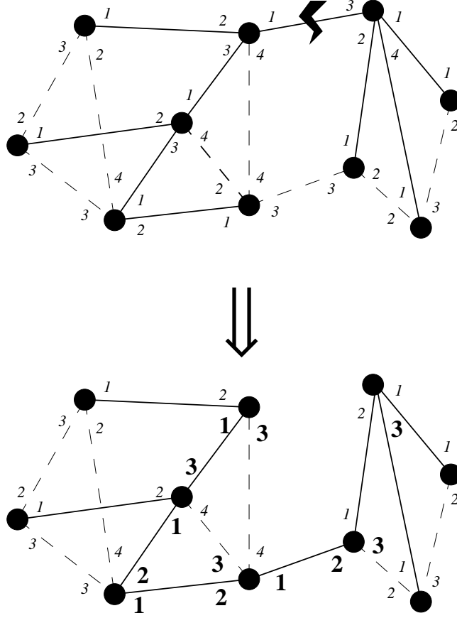
Figure 2: Removal of an edge belonging to the spanning tree.
