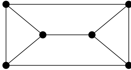
Figure 3: A graph in \mathcal{G}_3 \setminus \mathcal{G}_2
