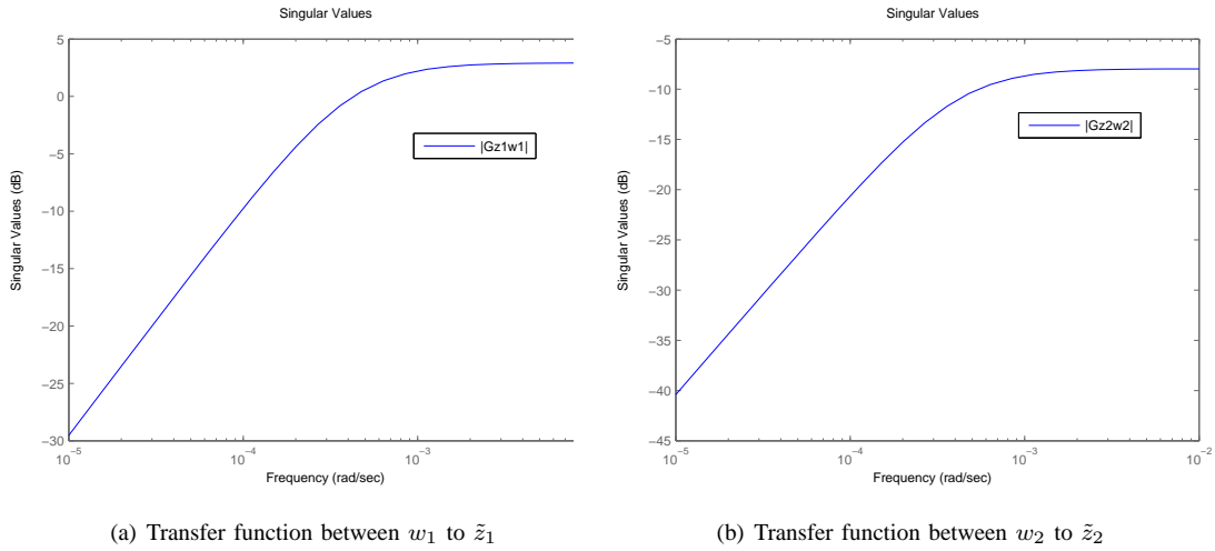
Fig. 1. Transfer function between w to \tilde{z}
