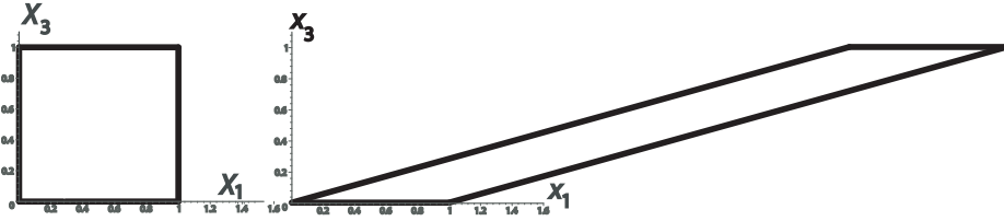
Figure 3: Large simple shear of a unit square in the surface of a semi-infinite incompressible neo-Hookean solid. When the solid is sheared by an amount K_0 \simeq 3.09 (Figure on the right), its surface wrinkles. The corresponding angle of shear is \tan^{-1} K_0 \simeq 72.0^\circ , which physically, is abnormally large. Then the wrinkles are parallel to the direction of greatest tension, which makes an angle \varphi_0 \simeq 16.5^\circ with the direction of shear (and so, the wrinkles are almost aligned with the sheared faces.)
