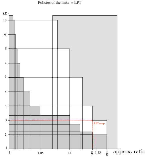
Fig. 4. Light grey (respectively Dark grey): Relation between \alpha and approximation ratios that it is possible (respectively it is not possible) to obtain if we wish an algorithm which returns \alpha -approximate Nash equilibria.
