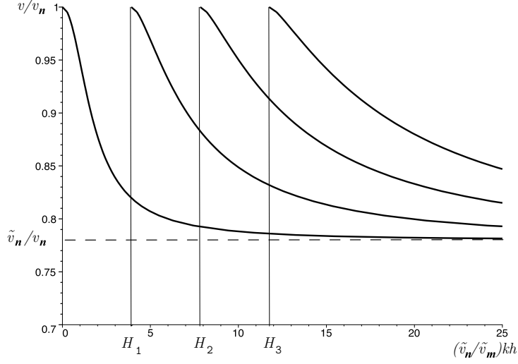
Figure 2: Dispersion curves for successive Love wave modes in a pre-strained configuration. Here H_l = l\pi/\sqrt{(c/\tilde{c})^2 - 1} , ( l = 1, 2, 3, 4, \dots ). Thus, for 0 < kh < (\tilde{v}_m/\tilde{v}_n)H_1 , only one mode may propagate (fundamental mode). For (\tilde{v}_m/\tilde{v}_n)H_l < kh < (\tilde{v}_m/\tilde{v}_n)H_{l+1} , l + 1 modes may propagate.
