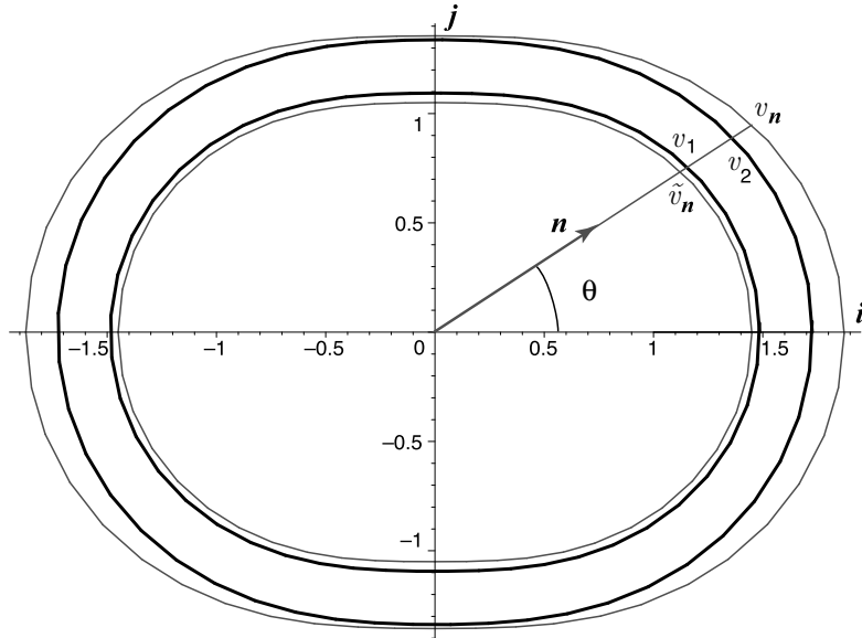
Figure 3: Polar graph of the Love wave speeds v_1 and v_2 corresponding to kh = \pi as a function of the angle \theta that the propagation direction \mathbf{n} makes with the direction \mathbf{i} .
