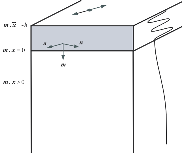
Figure 1: Sketch of the layered formation. The wave propagates in the direction of the unit vector \mathbf{n} , it is polarized along \mathbf{a} , and the magnitude of its amplitude varies along the direction of the unit vector \mathbf{m} , normal to the faces of the layer.
