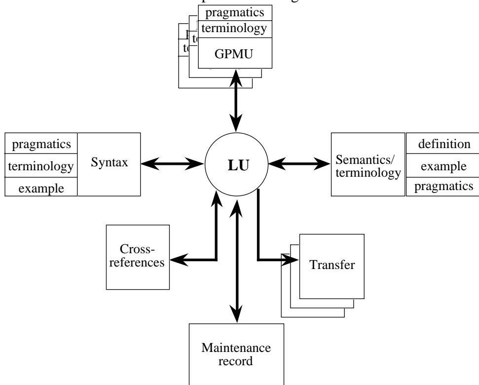
Figure 2: General view of a Lexical Unit.
