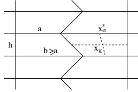
Fig. 1 Example of a trapezoidal mesh.
