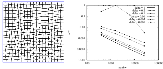
Fig. 2 Mesh of size n_x = 20 , and convergence of the L^2 error (erl2) for the MPFA O scheme for different values of \delta (nunkw denotes the number of cells n_x^2 ).
