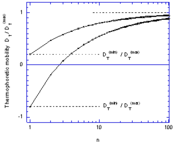
FIG. 2: Reduced thermophoretic mobility as a function of the chain length n . The points are calculated from Eq. (15) with \nu = 0.6 . The dashed lines indicate the maximum and minimum values where D_T^{(\max)} = \beta\varepsilon_p/(6\pi\eta a) and D_T^{(\min)} = D_T^{(\max)} - \beta\varepsilon_s/(\kappa\eta\ell) ; the latter may be positive or negative, depending on the relative magnitude of the two terms.
