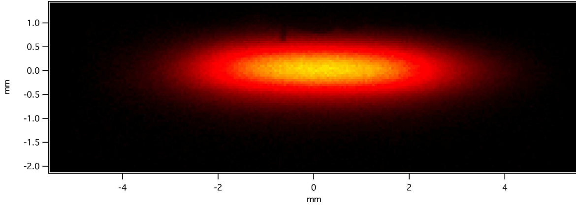
FIG. 3: Fluorescence image at \lambda = 422 nm of a trapped ion cloud (2 mm length and 200 \mu\text{m} width, FWHM) containing 3 \times 10^4 \text{Sr}^+ ions
