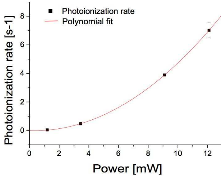
FIG. 5: Photoionisation rate as function of the average power of the ionisation beam. A perfect quadratic dependence is observed as expected for a two-photon absorption ionisation process.
