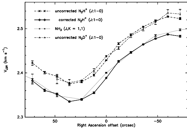
Fig. 3. N_2H^+ , N_2D^+ ( J:1-0 ) and NH_3 ( 1,1 ) line of sight velocity along the BB' cut (see Fig. 1). The N_2H^+ data are displayed with the original frequency (uncorrected) and with a correction of -41 \text{ m s}^{-1} . The uncorrected N_2D^+ ( J:1-0 ) points are consistent with the uncorrected N_2H^+ points despite the different opacities
