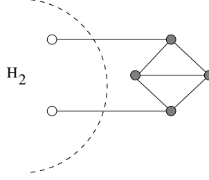
Fig. 2. The gadget for connecting half-edges
