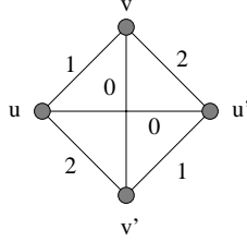
Fig. 1. Basic step of the induction
