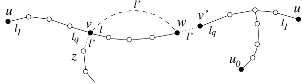
Fig. 1. Construction of G'' in the case where L' is not a palindrome. The dotted edges (v, z) and (w, v') are removed and the dashed edge (v, w) is added instead.
