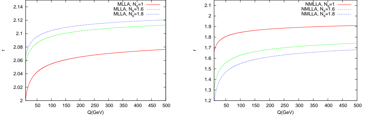
Figure 2: MLLA (18) and NMLLA (26) gluon to quark average multiplicity ratio as a function of Q = E\Theta in the vacuum ( N_s = 1 ) and in the medium ( N_s = 1.6 and N_s = 1.8 ).
