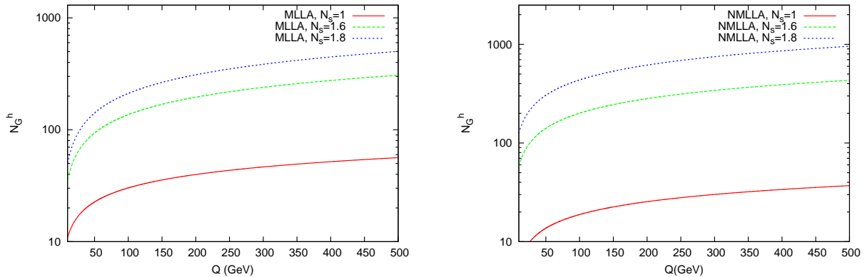
Figure 1: MLLA (13) and NMLLA (23) average multiplicity as a function of Q = E\Theta in the vacuum ( N_s = 1 ) and in the medium ( N_s = 1.6 and N_s = 1.8 ).
