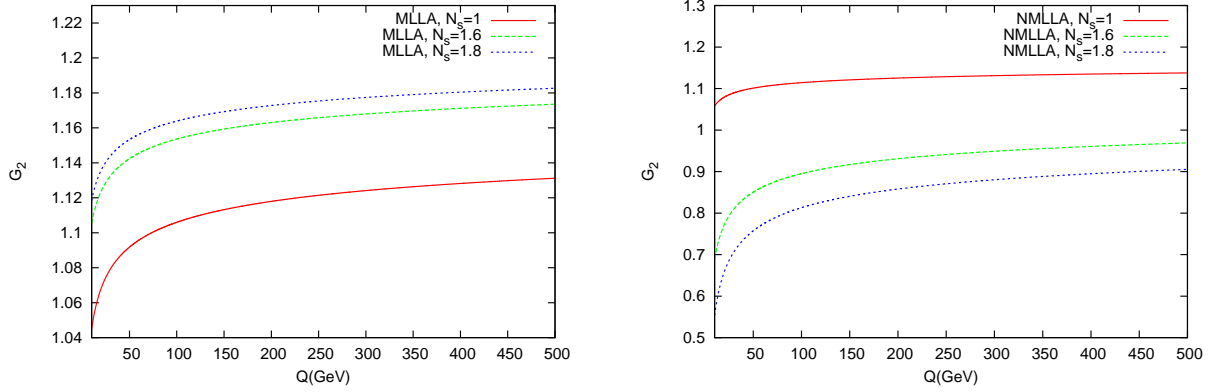
Figure 3: MLLA (38) and NMLLA (55) second multiplicity correlator inside a gluon jet as a function of Q = E\Theta in the vacuum ( N_s = 1 ) and in the medium ( N_s = 1.6 and N_s = 1.8 ).
