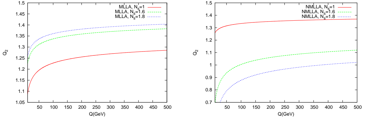
Figure 4: MLLA (41) and NMLLA (63) second multiplicity correlator inside a quark jet as a function of Q = E\Theta in the vacuum ( N_s = 1 ) and in the medium ( N_s = 1.6 and N_s = 1.8 ).
