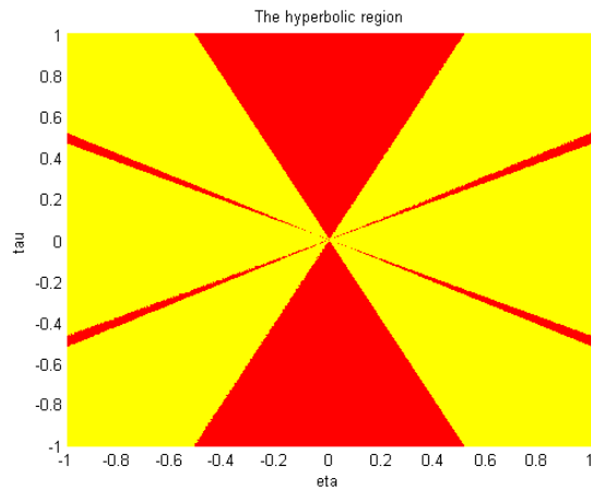
Figure 2: The hyperbolic region (in red) with six connected components for the fourth degree polynomial P in (10).
