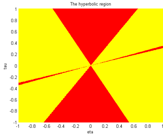
Figure 1: The hyperbolic region (in red) with four connected components for the third degree polynomial P in (8).
