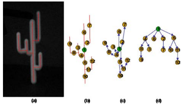
Figure 4: Graph construction from the skeleton
