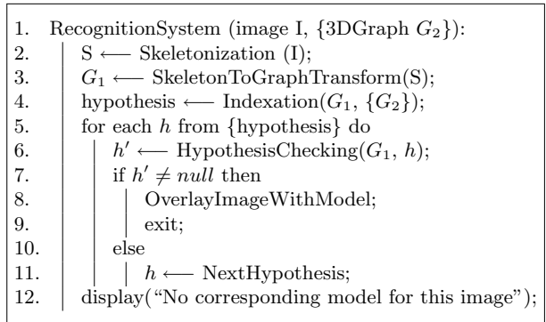
Figure 2: 2D/3D identification using skeletons
