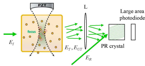
Figure 2. Principle of the PR detection of the acousto-optic signal. PZT: ultrasound transducer, E_I : illumination optical field; E_T, E_{UT} tagged or untagged field scattered by the sample; PR crystal: photorefractive crystal; L: lens that collect the scattered field into the crystal and photodiode; E_R : PR crystal reference (or pump) field.
