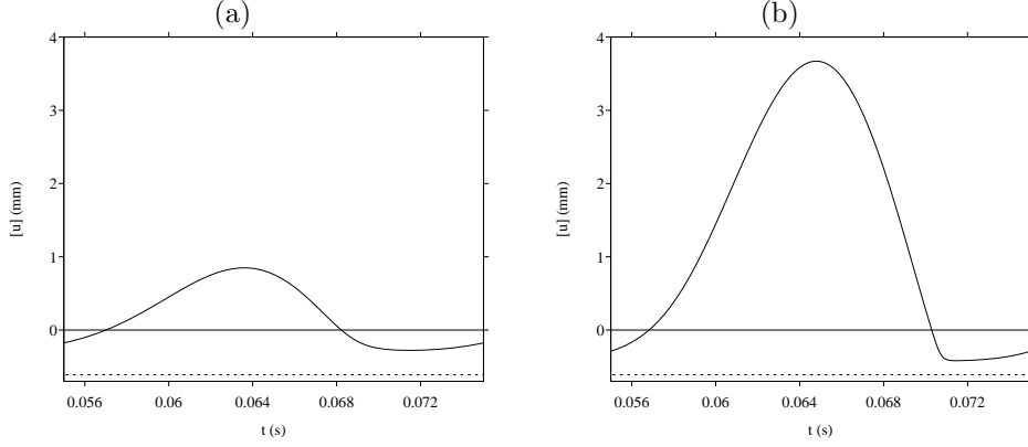
FIG. 2.4. Time history of [u(\alpha, t)] , at two incident elastic velocities: v_0 = 0.2 m/s (a) and v_0 = 0.5 m/s (b). The horizontal dotted line denotes -d .
