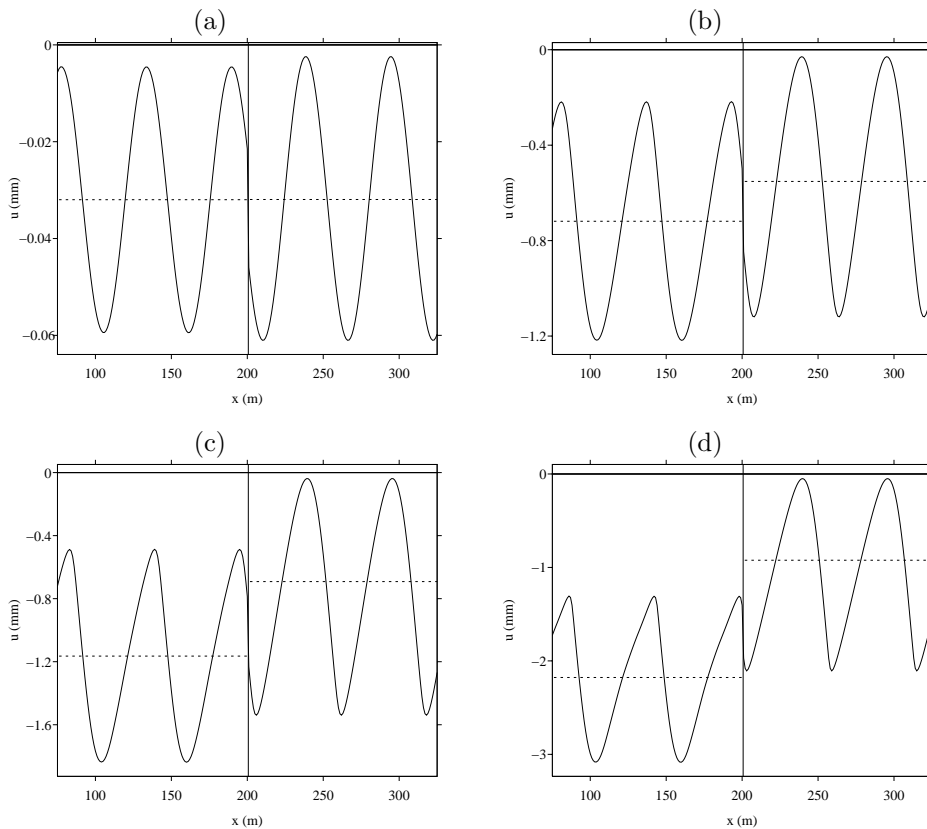
FIG. 2.3. Model 1 (2.7): snapshots of the elastic displacement, for various amplitudes v_0 of the incident elastic velocity: 0.01 m/s (a), 0.2 m/s (b), 0.3 m/s (c) and 0.5 m/s (d). The vertical solid line denotes the location \alpha = 200 m of the crack. The dotted horizontal lines denote the mean value of the elastic displacement on both sides of \alpha .
