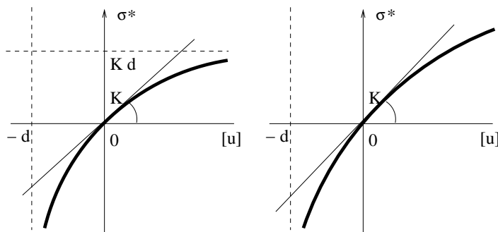
FIG. 2.2. Nonlinear relation between the stress and the jump of the elastic displacement at \alpha . Left row: model 1 (2.7), right row: model 2 (2.8).
