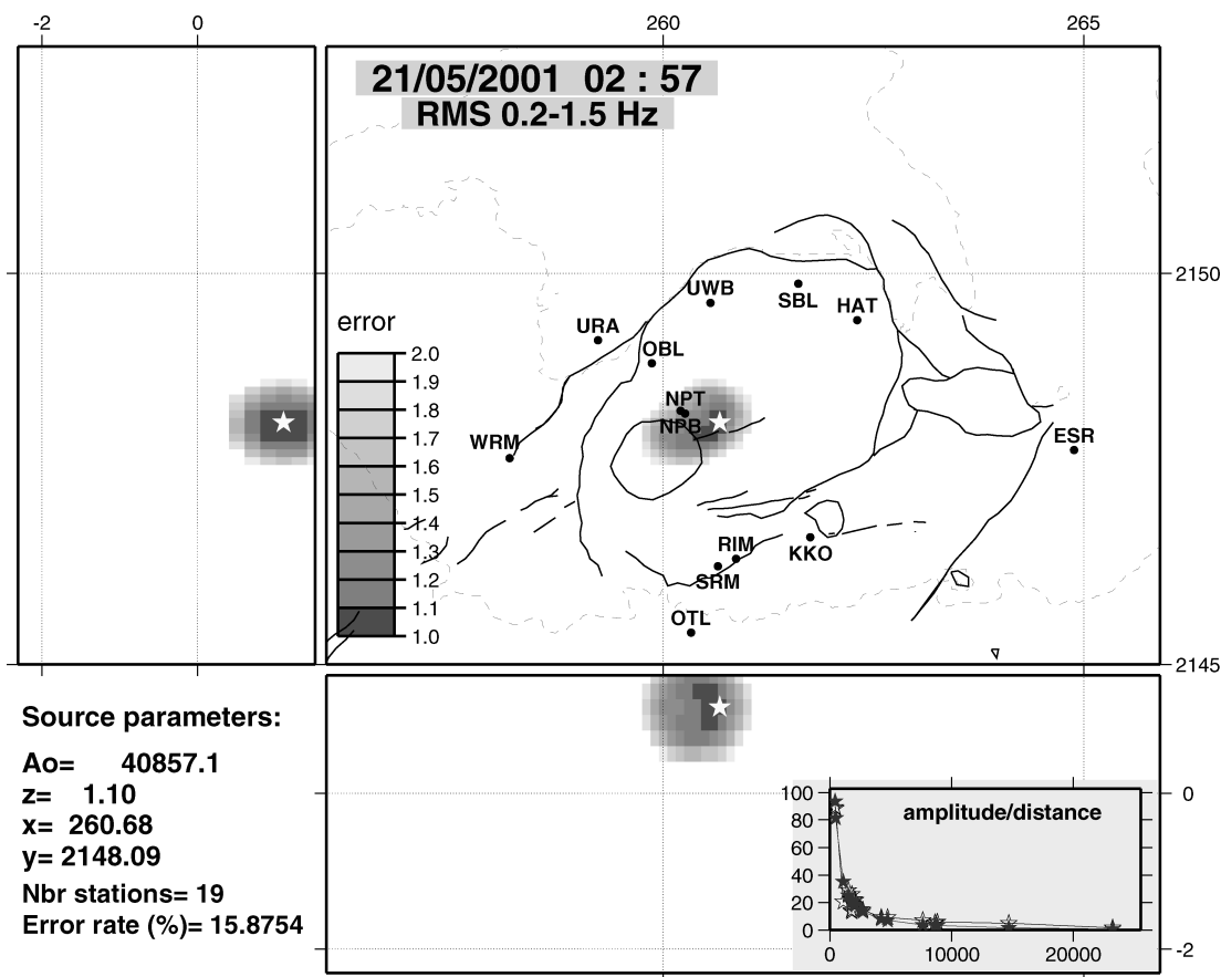
Figure 2. Source location for the LP event, obtained by inverting the spatial distribution of seismic amplitudes calculated peak to peak. Source location (white star) and its error (grey scale) are plotted both for the horizontal projection and for the north–south and the east–west vertical cross sections. The figure shows the station locations (black dots), as well as the Caldera border and the main geological features. The retrieved source parameters are indicated in the bottom left-hand corner and the fit of the seismic amplitude versus epicentral distance is given in the bottom right corner: empty stars represent the observations and black stars represent the calculated amplitudes.
