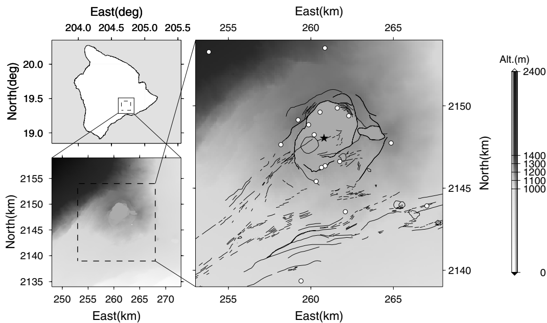
Figure 3. Area of study. Top left-hand panel: map of the Big Island of Hawaii showing the area of the study: the continuous line represents the 25 \times 25 km area including the absorbing boundary, while the dashed line corresponds to the inner 15 \times 15 km area. Bottom left-hand panel: enlarged plot of the area under study, topography is represented in tones of grey (the scale is plotted on the right side of the figure). Right-hand panel: enlarged plot of the inner area, showing the topography (tones of grey), the major fractures and geological features, including Kilauea caldera border and the inner Halemaumau crater (black lines), as well as station locations (white circles) and the epicentral location of LP event (black star).
