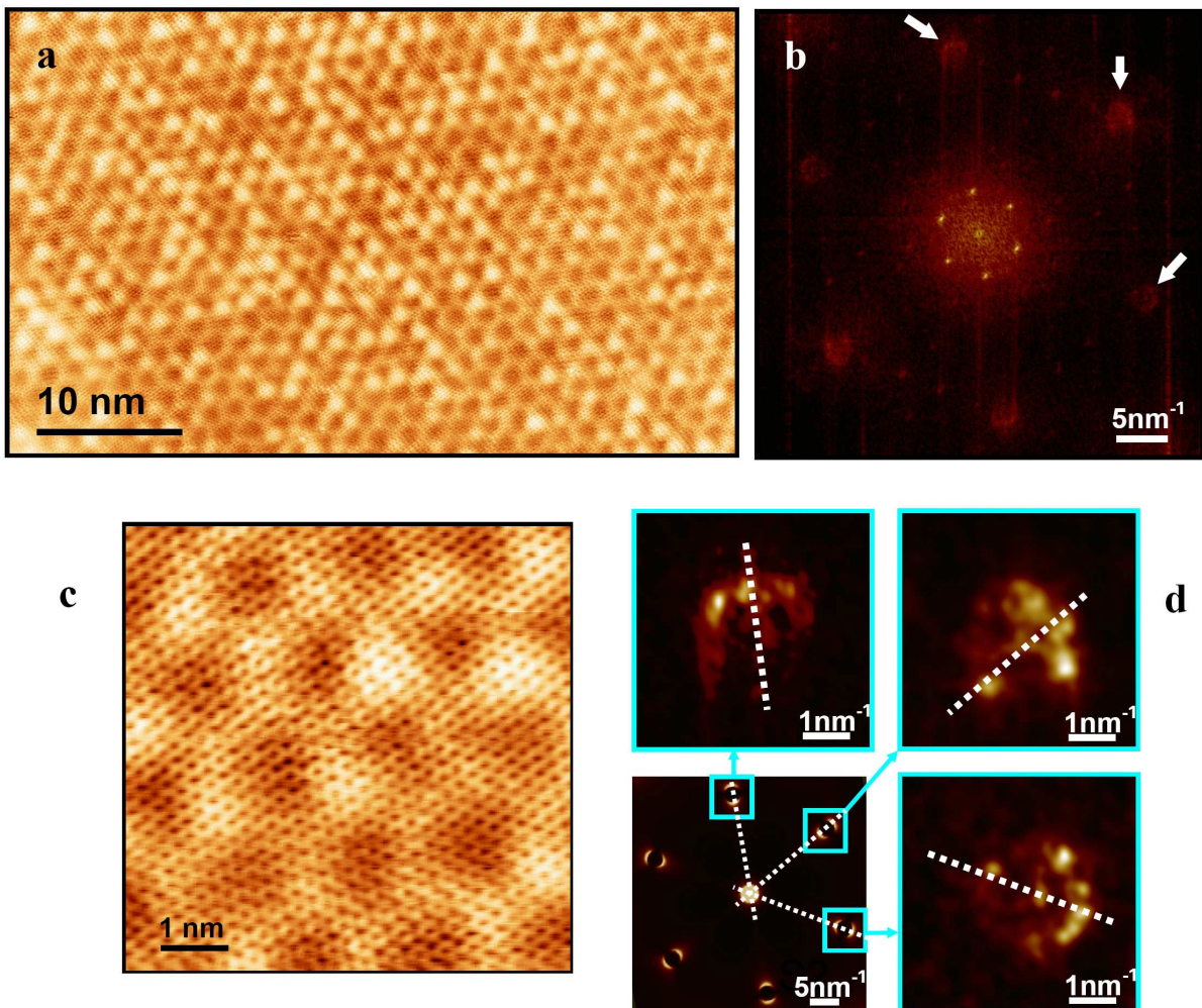
Fig. S2. STM analysis of the quantum interferences related to intervalley scattering in graphene monolayer. (a) 30 \times 50 \text{ nm}^2 image of a monolayer terrace at 4.5 K, sample bias: -2 mV, tunnelling current: 0.4 nA. (b) Fast
