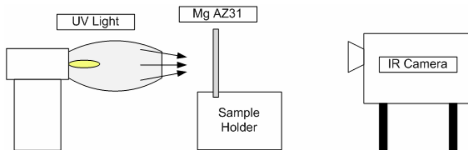
Figure 1: Selective annealing experimental setup
