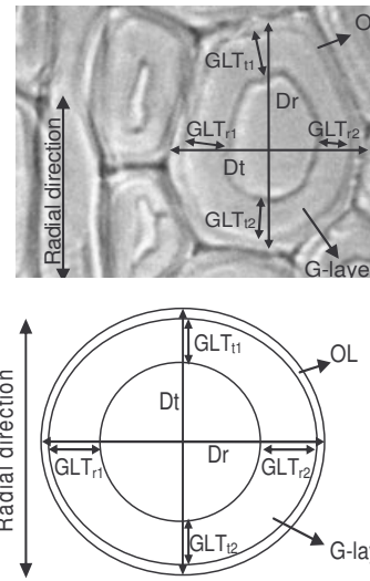
Fig. 3. Detail of figure 2 presenting the G-layer thickness and cell diameter measurements. G-layer thickness was always measured in the same 4 positions (2 radial: (GLT r1 , GLT r2 ) and 2 tangential: (GLT t1 , GLT t2 )). Cell diameter was measured in 2 directions (radial: Dr and tangential: Dt).
