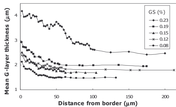
340 Fig. 1. Mean G-layer thickness ( MGLT , \mu m ) variation with the distance from the border for 5 samples with different GS values.
