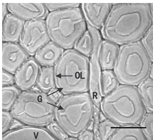
Fig. 2. Transverse section of sample 1. G: G-layer; OL: other cell wall layers including compound lamella, S 1 and S 2 ; V: vessel; R: ray. Scale bar = 20µm.
