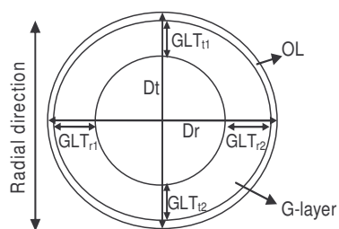
Fig. 3. Detail of figure 2 presenting the G-layer thickness and cell diameter measurements. G-layer thickness was always measured in the same 4 positions (2 radial: (GLT r1 , GLT r2 ) and 2 tangential: (GLT t1 , GLT t2 )). Cell diameter was measured in 2 directions (radial: Dr and tangential: Dt).
