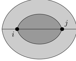
FIGURE 28. Case 4: i and j belong to V_c .
