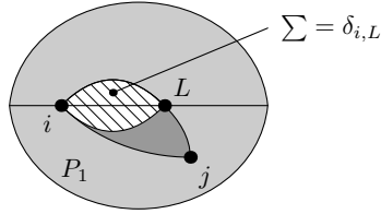
FIGURE 27. Case 3: i \in V_c and j \notin V_c .
