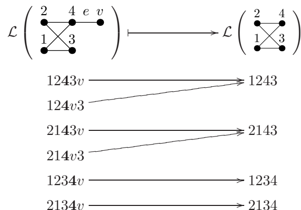
FIGURE 7. Example of the map er_v
