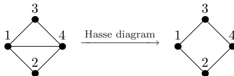
FIGURE 4. Example of a poset and his Hasse diagram.
