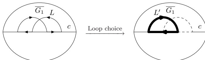
FIGURE 20. Good choice of cycle
