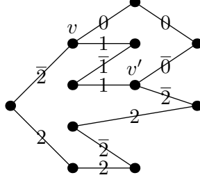
FIGURE 11. Example of a graph G with cyclomatic number 2.
