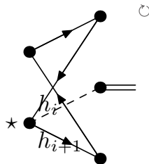
FIGURE 17. Example of a rooted map M' with an admissible cycle of type 2.
