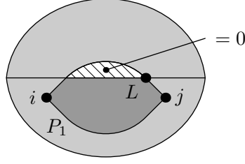
FIGURE 26. Case 2: i \notin V_c and j is in the same region than i .
