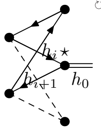
FIGURE 15. Example of a rooted map M with an admissible cycle of type 1.
