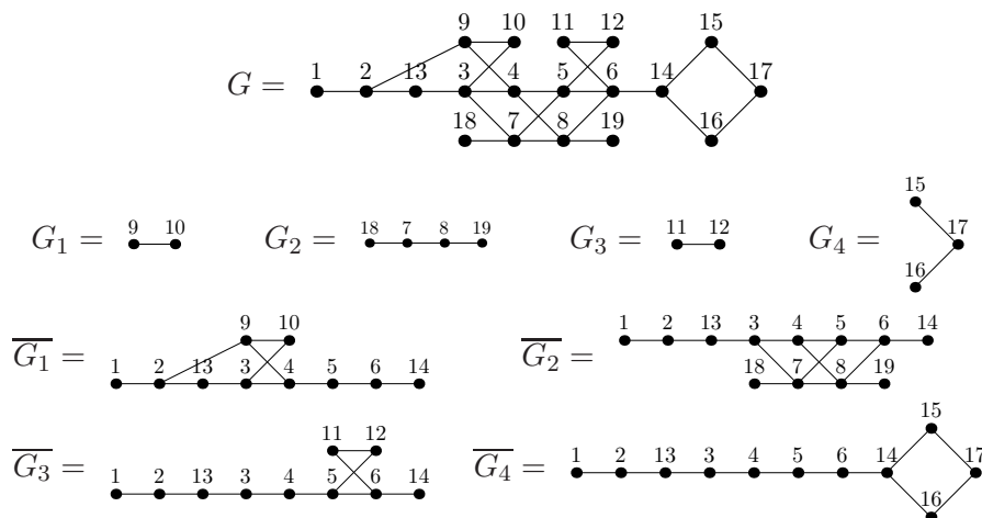
FIGURE 19. A graph G with a chain c , the components G_i of G \setminus c and the corresponding regions \overline{G}_i .
