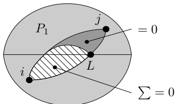
FIGURE 25. Case 1: i \notin V_c and j is not in the same region than j .
