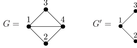
FIGURE 5. G' is the induced graph of G by \{1, 2, 3\} .
