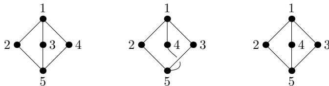
FIGURE 14. Example of three different maps.
