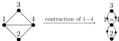
FIGURE 6. Example of contraction.
