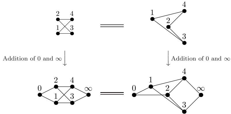
FIGURE 22. The graph G is planar, but not strongly planar.
