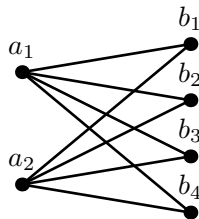
FIGURE 12. The bipartite graph G_{2,4} .
