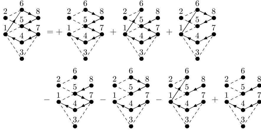
FIGURE 8. Example of application of theorem 4.1
