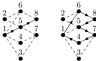
FIGURE 3. Example of a chain and a cycle C (we recall that orientations are from left to right).
