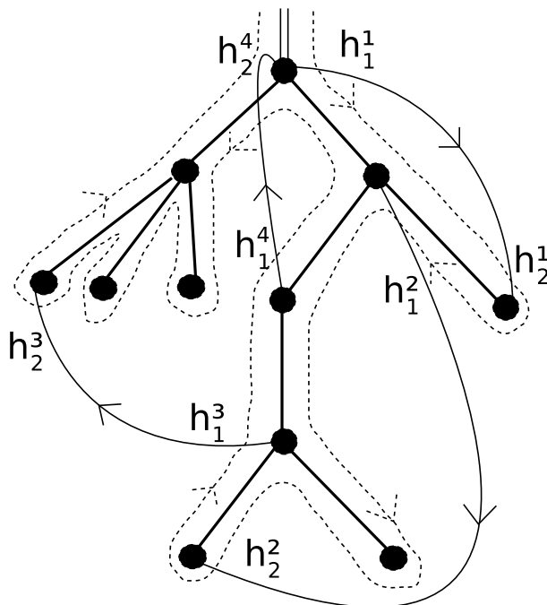
FIGURE 18. Tour of a spanning tree of a map.
