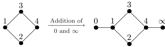
FIGURE 21. The graph G is strongly planar.
