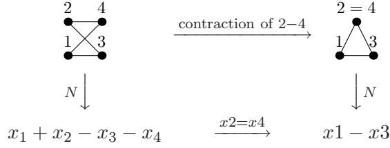
FIGURE 9. Contraction and numerator
