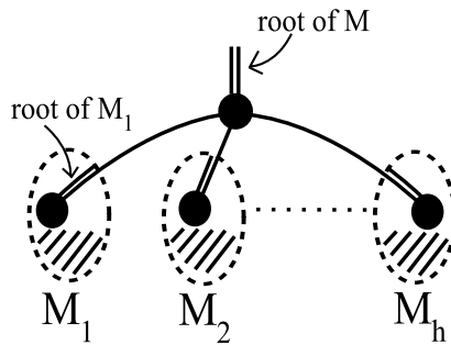
FIGURE 16. A generic rooted map M without admissible cycles of type 1
