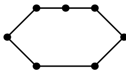
FIGURE 23. A diamond
