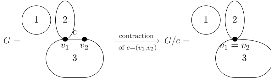
FIGURE 10. The different cases of the proof of proposition 4.6
