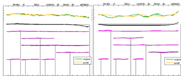
Figure 1. Comparing original and predicted prosodic contours for the sentence “llevaba el típico conjunto de blusas de quitaipón ». Left: f0 contours. Right: syllable lengthening. For each caption: top: superposition of predicted (yellow) and original (green) contours; bottom: elementary contours predicted for each discourse function; the prediction is obtained by superposing and adding these elementary contours. Horizontal axis represents the syllable count.
