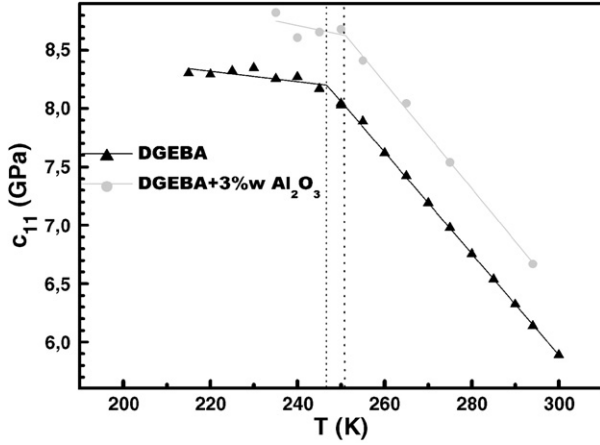
Fig. 6. Evolution of the elastic constant c_{11} (Young's modulus) versus temperature for pure DGEBA (triangles) and nanocomposites (circles).
