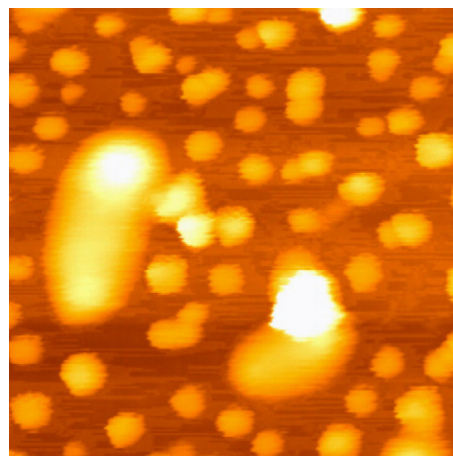
Fig. 4. IC-AFM image of \text{Fe}(\text{IO}_3)_3 nanocrystals dispersed on HOPG ( 1 \times 1 \mu\text{m}^2 , grey scale 100 nm).
