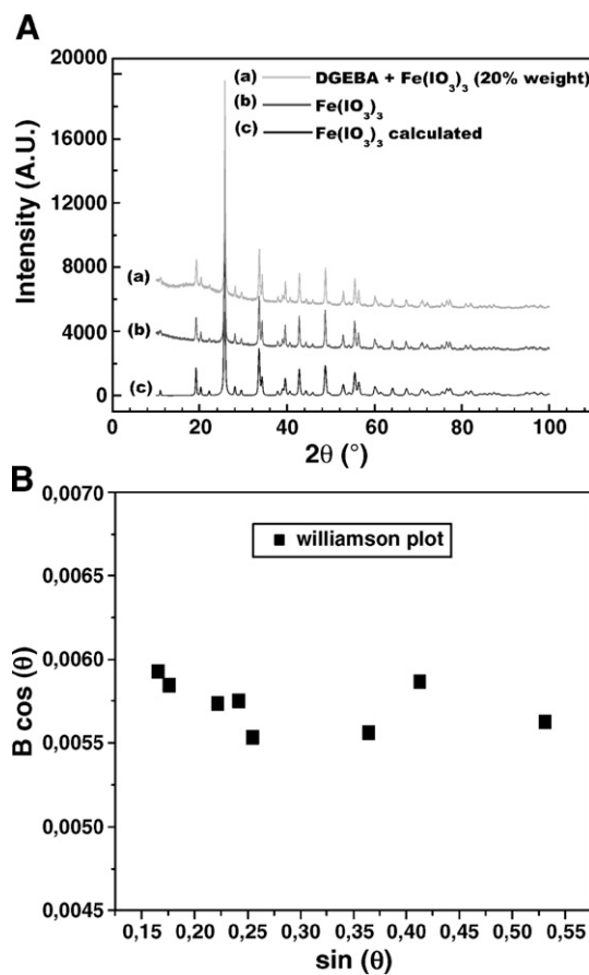
Fig. 1. A: X-ray diffraction patterns of \text{Fe}(\text{IO}_3)_3 . (a) Embedded in a DGEBA matrix, (b) observed on nanopowders and (c) calculated from the single crystal data. B: Williamson plot corresponding to the XRD pattern of \text{Fe}(\text{IO}_3)_3 nanopowders.
