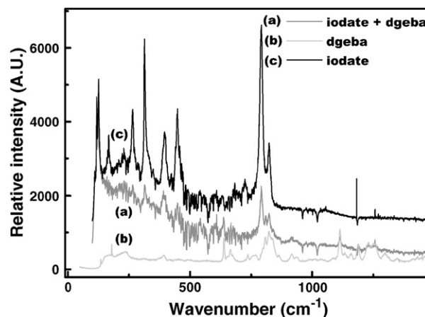
Fig. 5. Raman spectrum of nanocomposite DGEBA/ \text{Fe}(\text{IO}_3)_3 nanoparticles (a), compared to those of pure DGEBA (b) and \text{Fe}(\text{IO}_3)_3 nanoparticles (c).
