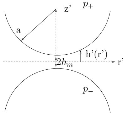
Figure 1: Slide view of the two identical particles under study.
