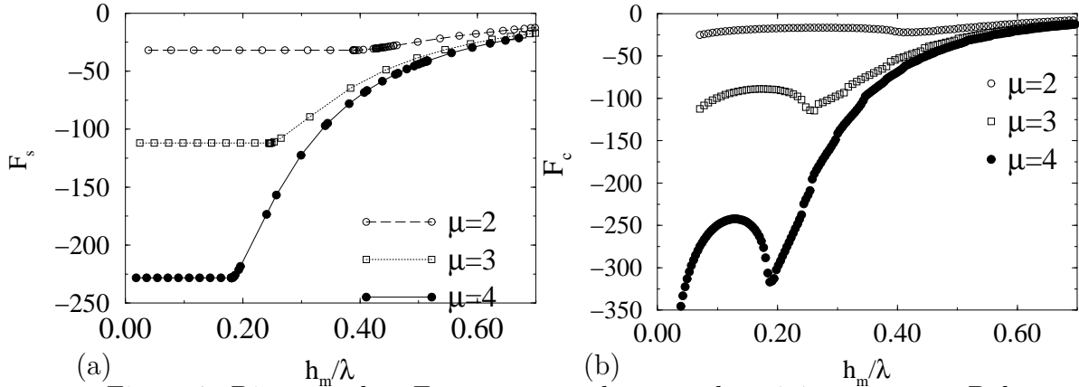
Figure 3: Dimensionless Force computed versus the minimum-gap to Debye layer ratio for different value of the mixed boundary condition parameter \mu . (a) Between two spheres, (b) between two cylinders.
