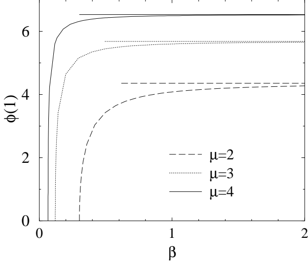
Figure 2: Surface potential of an anti-symmetric solution \phi(1) at \zeta = 1 versus dimensionless parameter \beta . The dotted lines display an asymptotic value which can be computed ( Cf [Plouraboué and Chang(2008)] for more details on this point).
