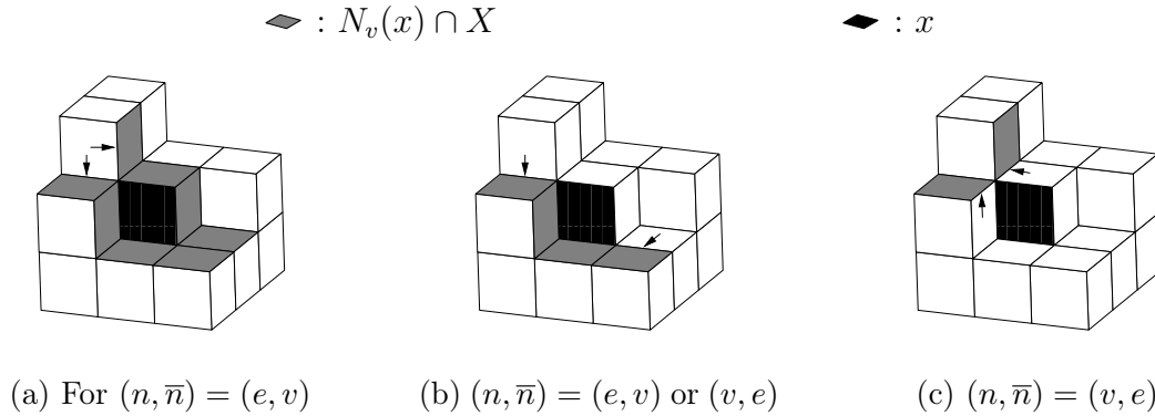
Fig. 13. Border edgels associated with an n_x -connected component of G_n(x, X) .
