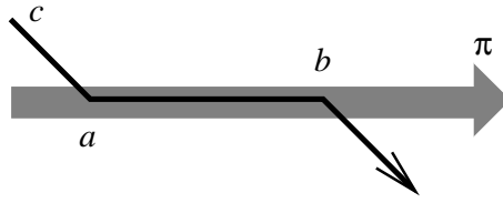
Fig. 6. There are two ways to check that c crosses \pi from left to right.
