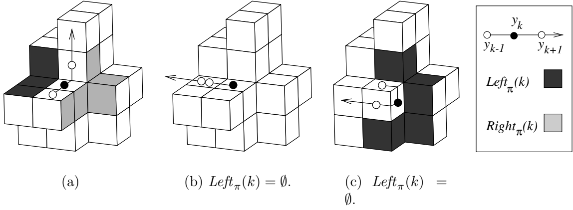
Fig. 3. Some illustrations of the sets Left_\pi(k) and Right_\pi(k) where \pi = (y_k)_{k=0, \dots, p} .
