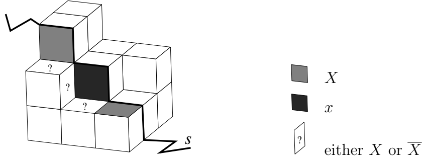
Fig. 12. If the two grey surfels belong to the same v_x -connected of G_v(x, X) it is clear that \text{Card}(\mathcal{C}_v^x[G_v(x, X)]) = 1 and \text{Card}(\mathcal{C}_e^x[G_e(x, \bar{X})]) = 1 .
