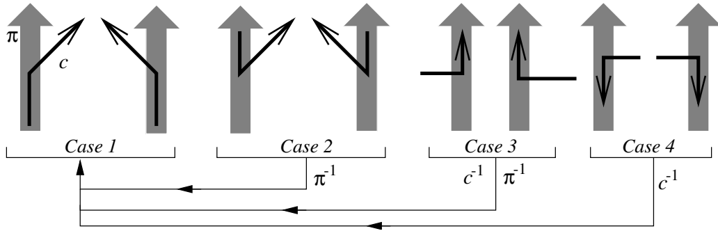
Fig. 7. An illustration of the cases investigated in the proof of Lemma 8 when \{x_{i-1}, x_{i+1}\} \cap \{y_{k-1}, y_{k+1}\} \neq \emptyset
